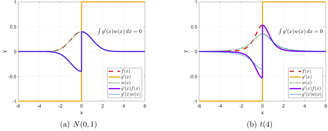
Figure 1: g_h(x) = \beta_0 x + |x| (with \beta_0 = 0 )
