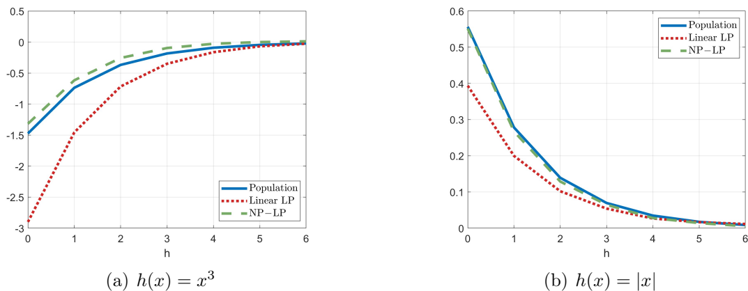
Figure 5: Comparison of LP with local linear, GEV distribution.
