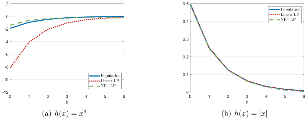
Figure 4: Comparison of linear LP and local linear, t_4 distribution.
