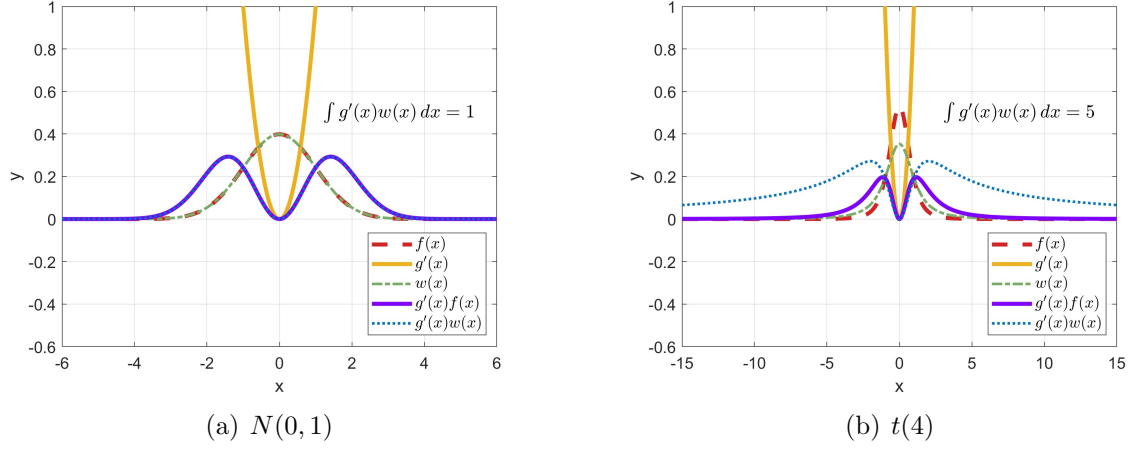
Figure 2: g_h(x) = \beta_0 x + \frac{1}{3}x^3 (with \beta_0 = 0 )
