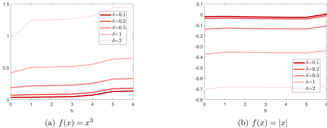
Figure 6: Percentage bias of LP relative to population ARF, N(0,1) distribution.
