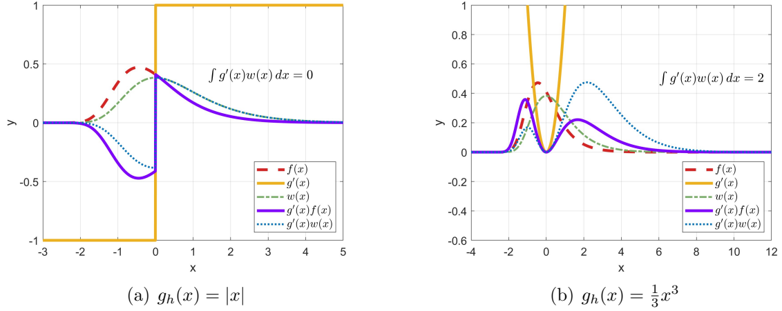
Figure 3: f(x) is GEV(0, 1, 0)
